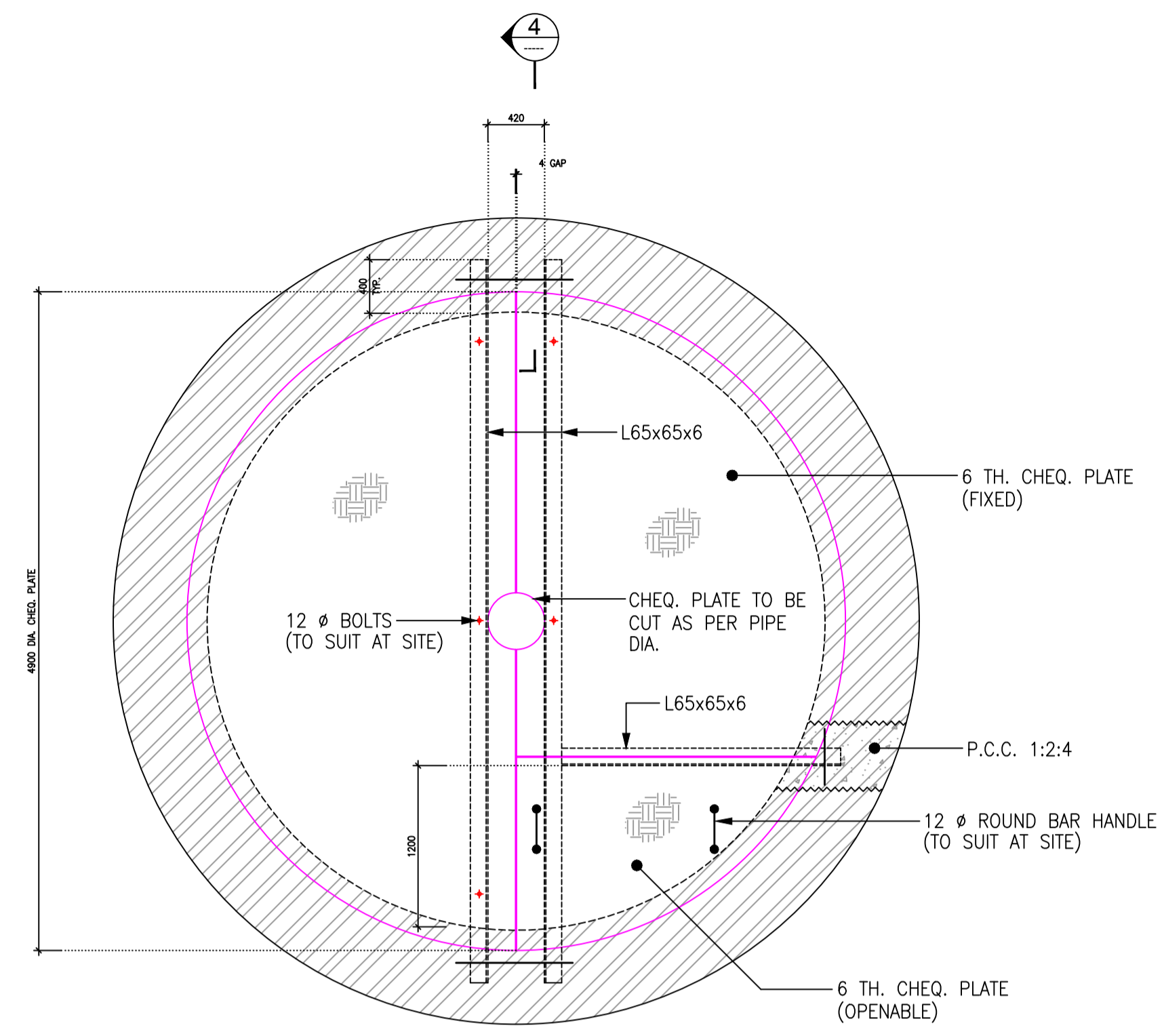
3 DETAILS OF TOP COVER SCALE 1:25
