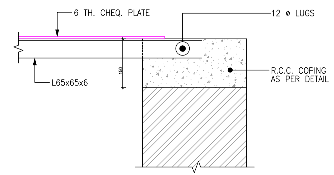
4 SECTION SCALE 1:10
