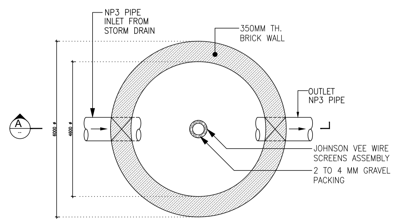
1 PLAN OF PERCOLATING WELL SCALE 1:50
