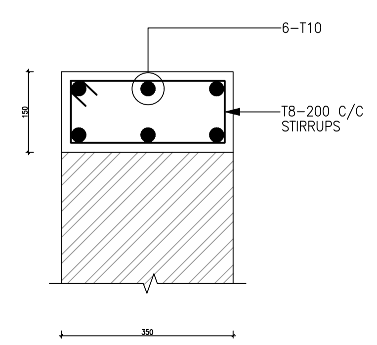
5 DETAILS OF R.C.C. COPING SCALE 1:10
