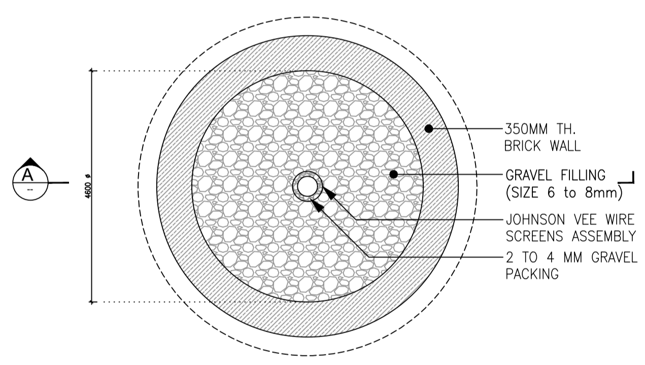
2 PLAN OF PERCOLATING WELL SCALE 1:50
