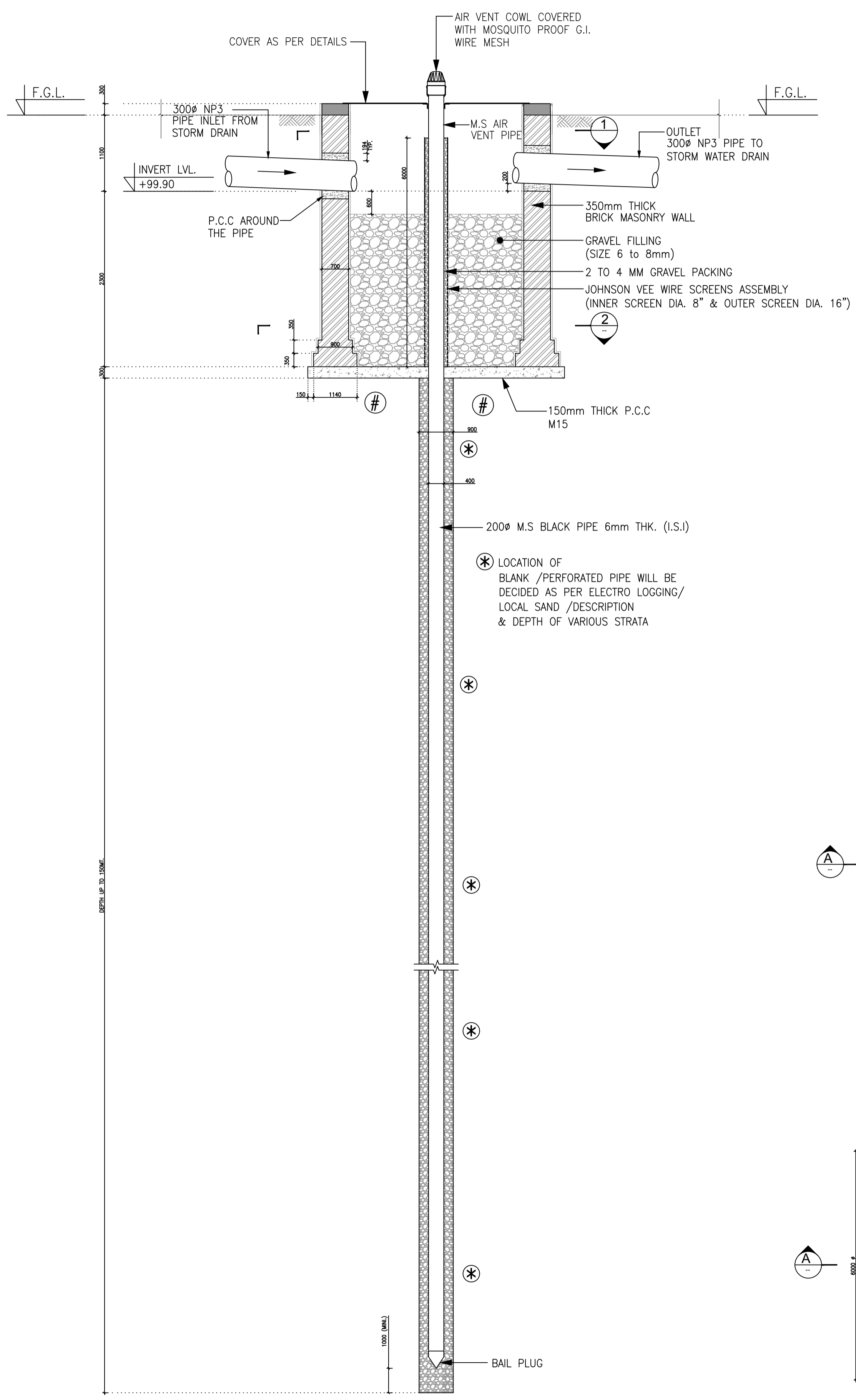
A SECTION THROUGH WELL (R.W. -02 TO R.W. -17) SCALE 1:50
