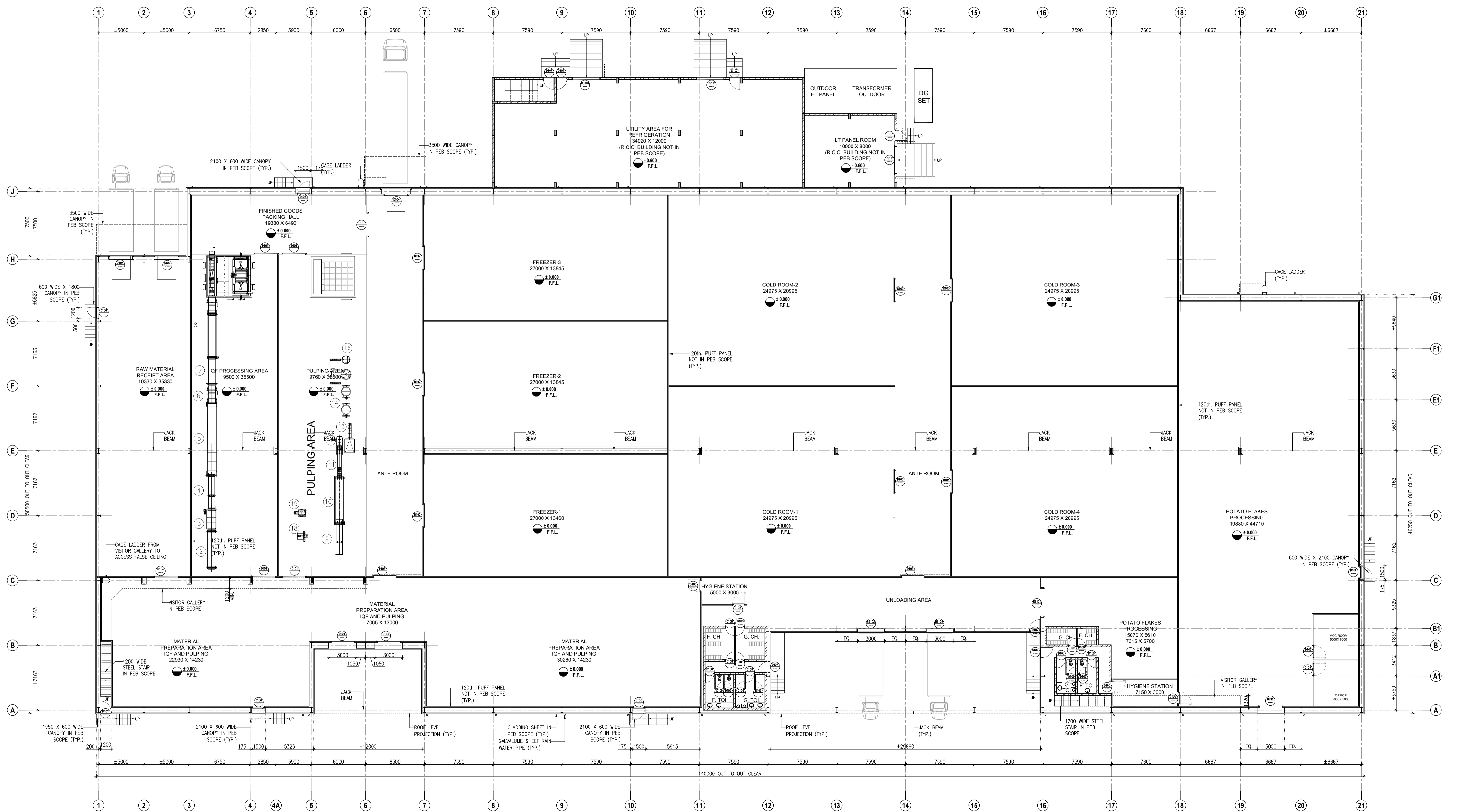
1 GROUND FLOOR PLAN SCALE 1:200
