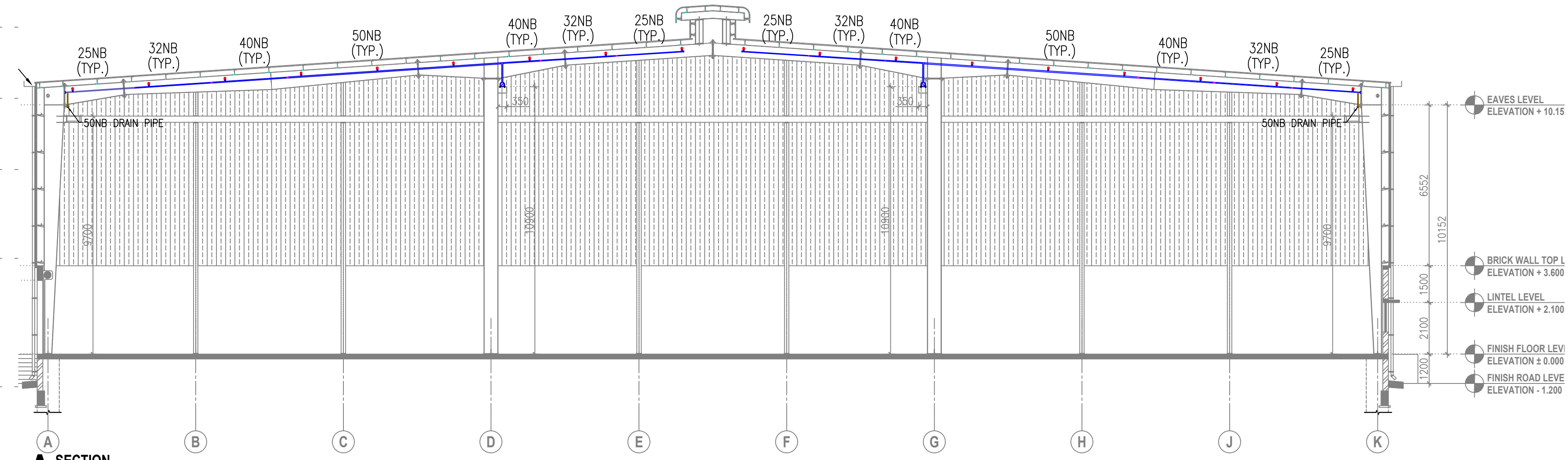
A SECTION SCALE 1:150
